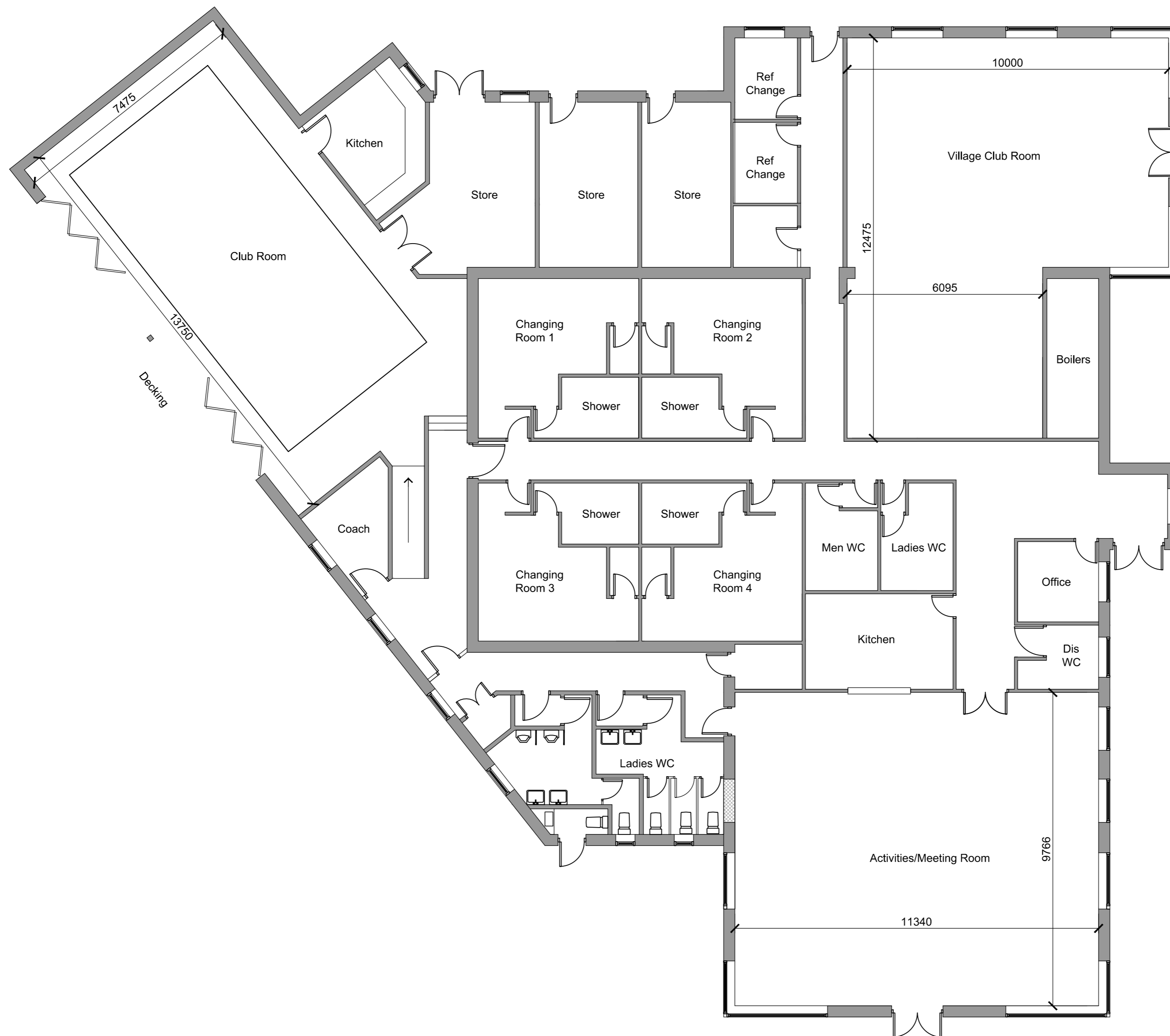
Jubilee Fields Pavilion - Proposed Floor Plan Scale 1:100
