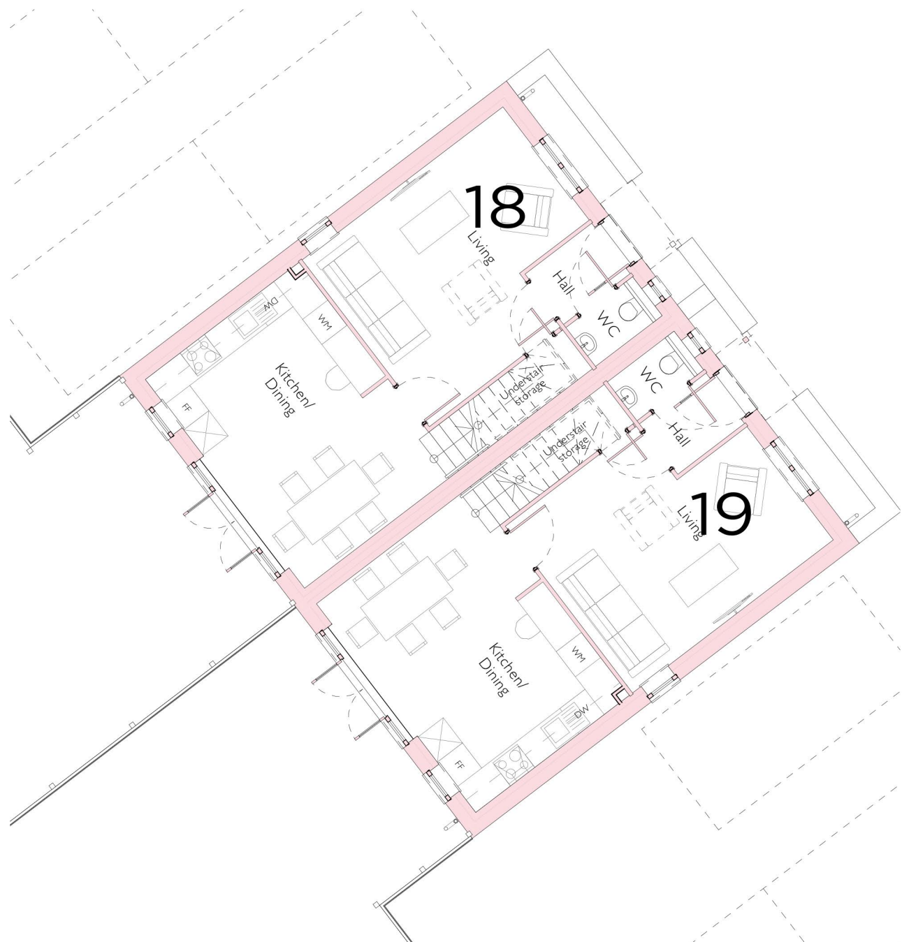
Ground Floor 1:100
