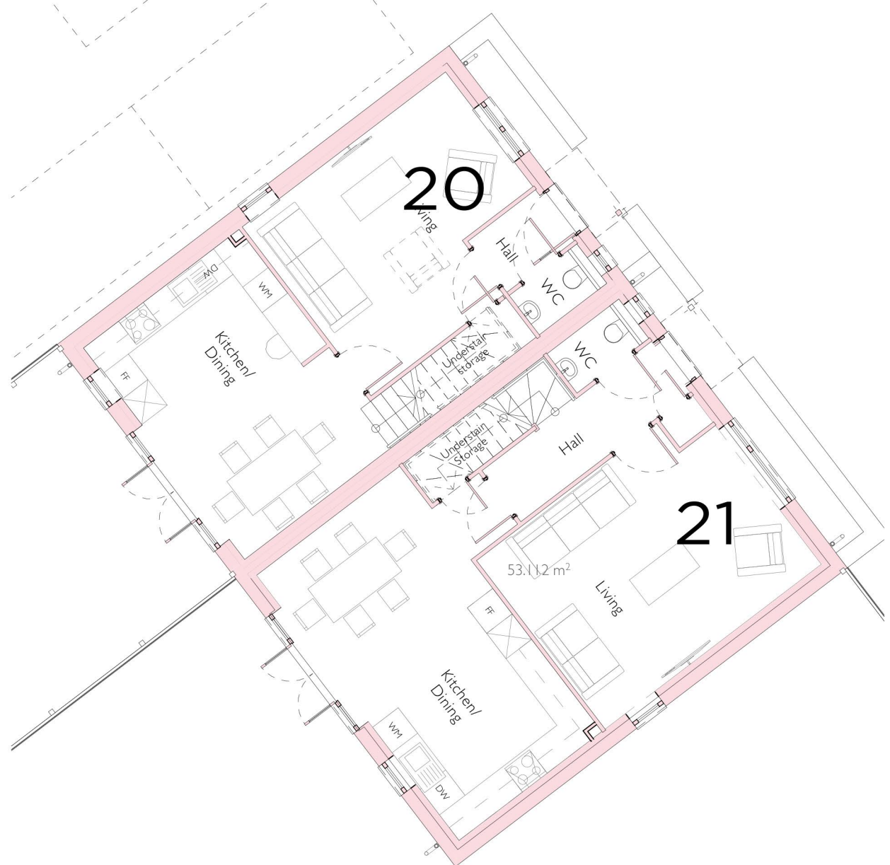
Ground Floor 1:100
